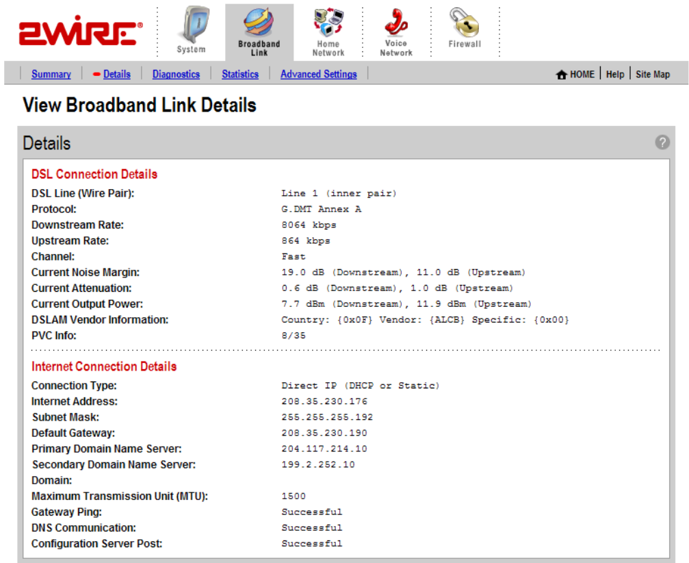
Figure 8. View Broadband Link Details Page
