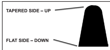
GASKET ORIENTATION
