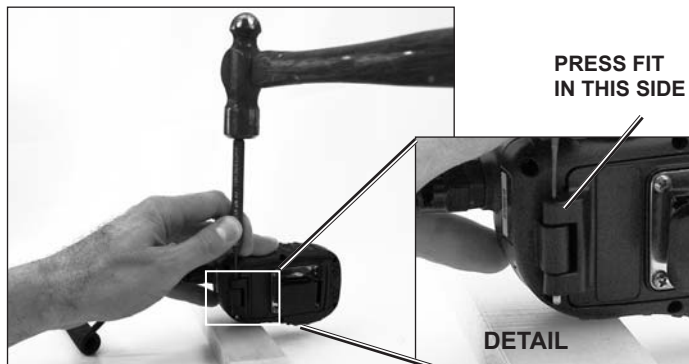
BATTERY DOOR REMOVAL
