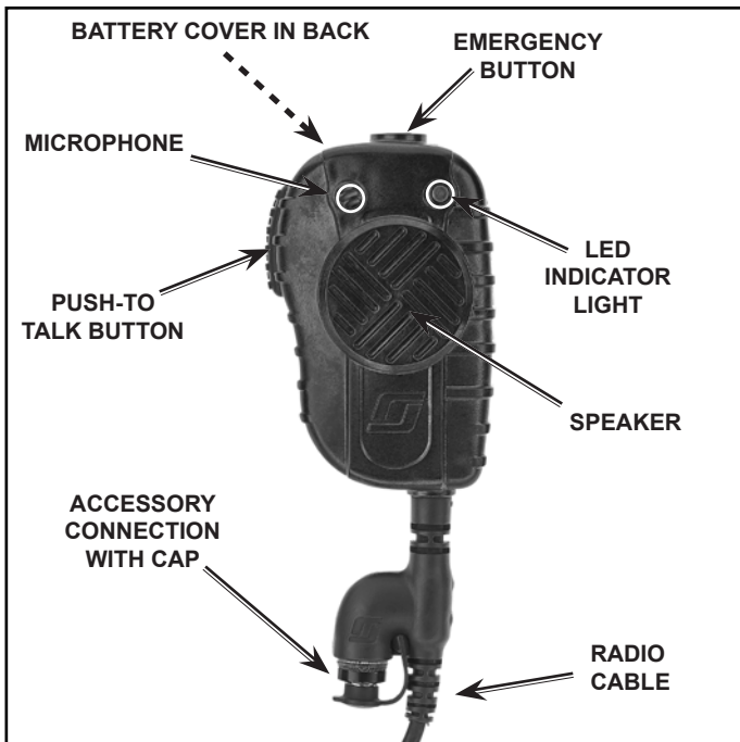
EPIC 3 BLUETOOTH LSM
