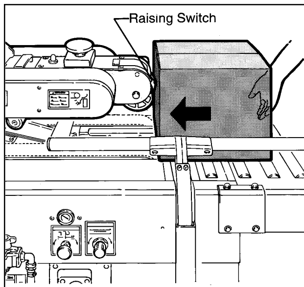
Figure 3-8 – Drive Assembly Raising Switch
