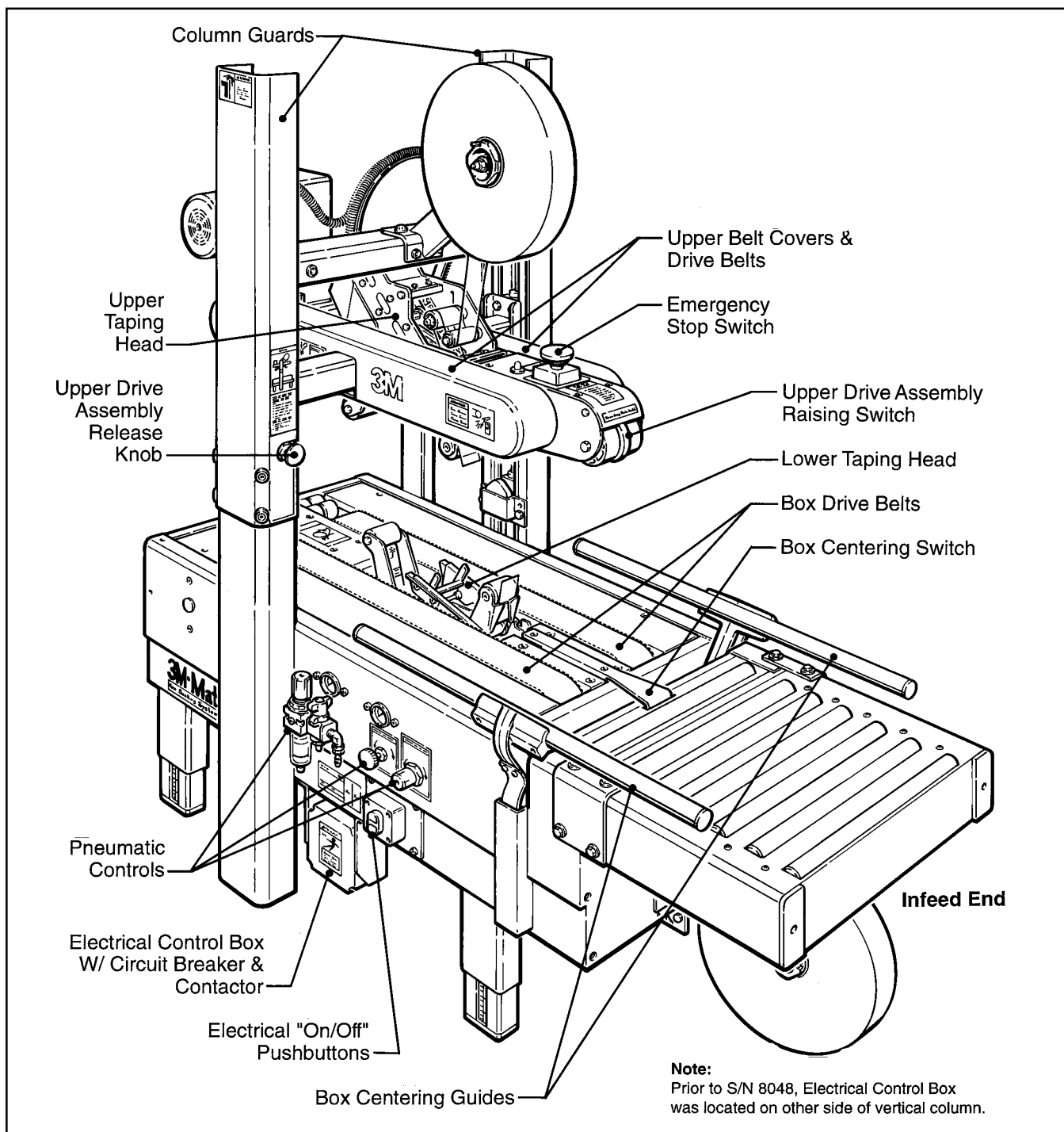
Figure 3-1 – 700r3 Case Sealer Components (Left Front View)
