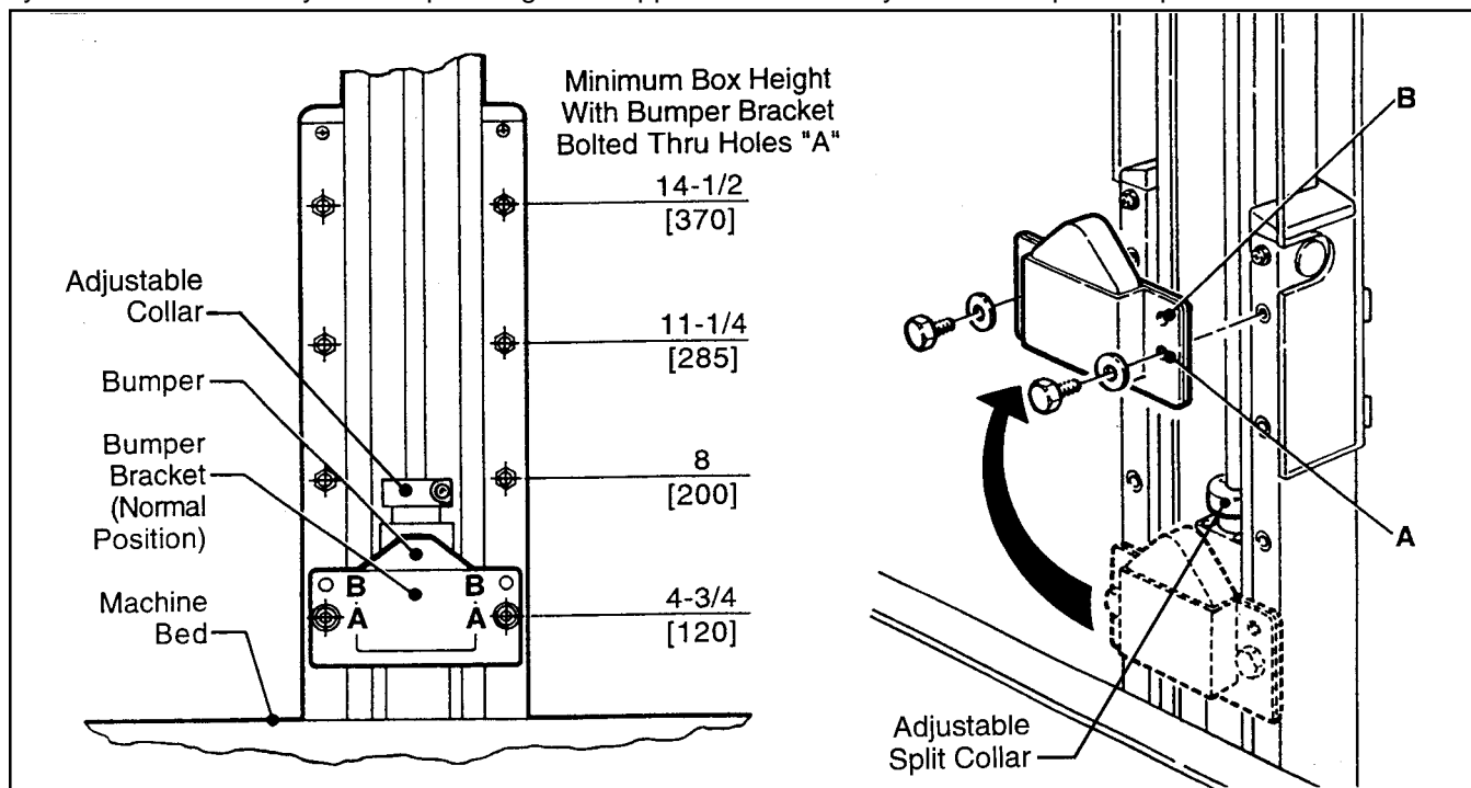
Figure 6-5 – Stop Bumpers
