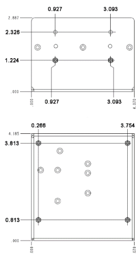
Figure 102: 3e-523N Mounting Dimensions
