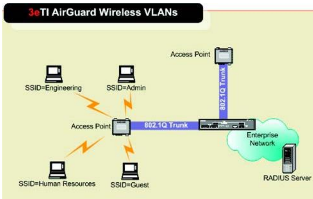
Figure 13: Wireless VLAN Communications
