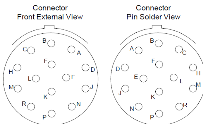
Figure 6: AUX Port Pin Definition
