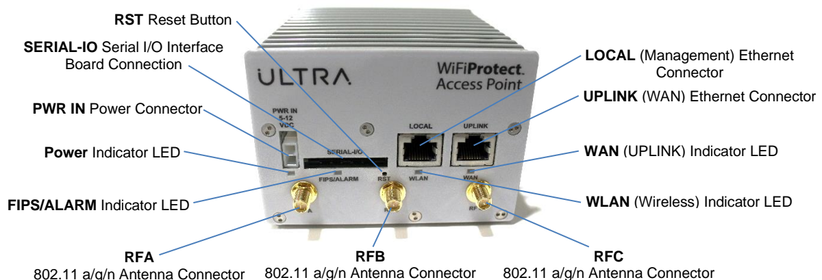
Figure 2: 3e-523 External Connectors and Indicators
