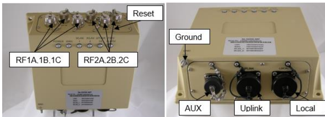
Figure 5: 3e-525N External Interfaces
