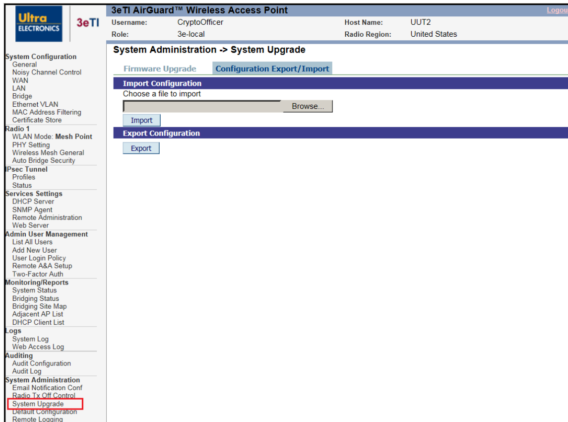
Figure 91: System Administration – System Upgrade – Configuration Export/Import
