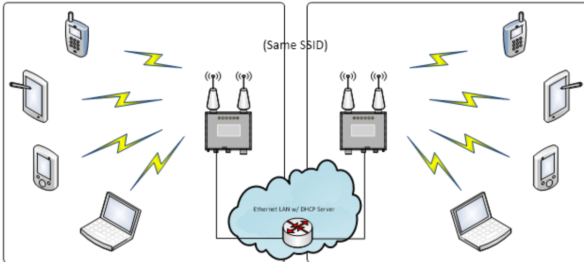
Figure 10: Multiple APs Connected to an Existing Ethernet Network with DHCP Server
