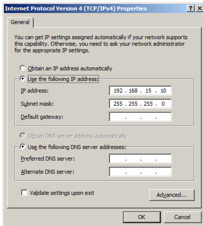
Figure 15: Local PC IP Address Configuration
