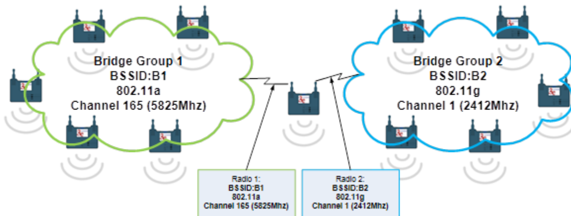
Figure 11: Dual Bridge Configuration
