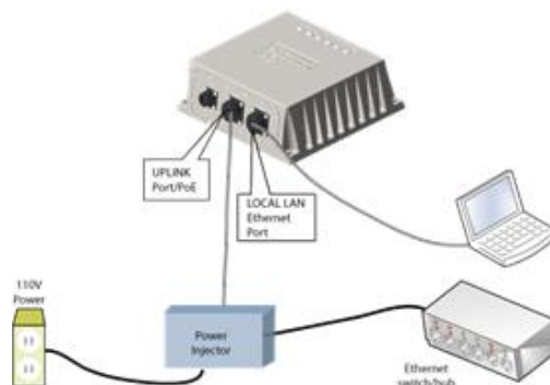
Figure 14: 3e-525N Quick Setup
