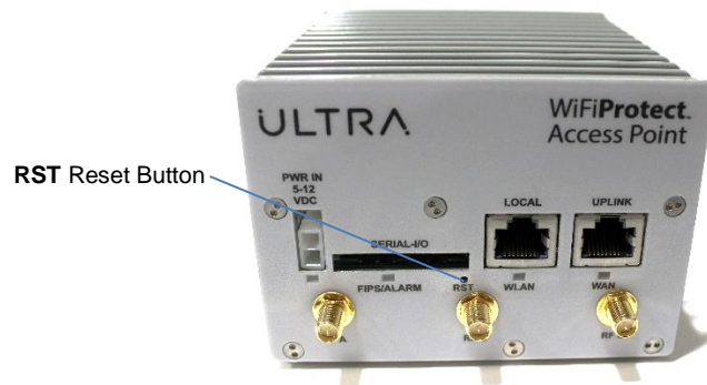
Figure 4: 3e-523N External Connectors and Indicators
