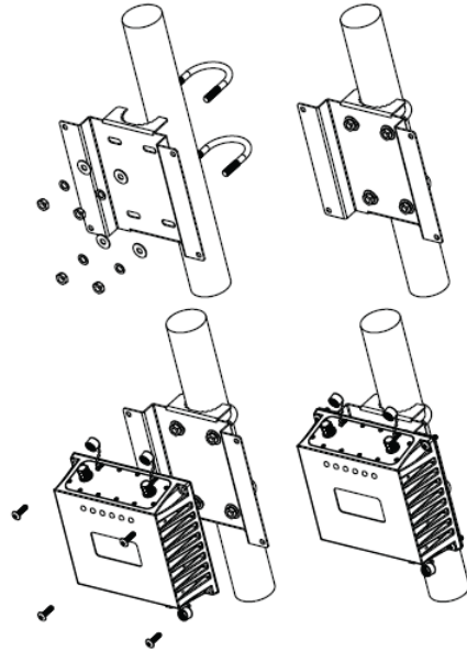
Figure 104: 3e-525N Pole Mount Installation
