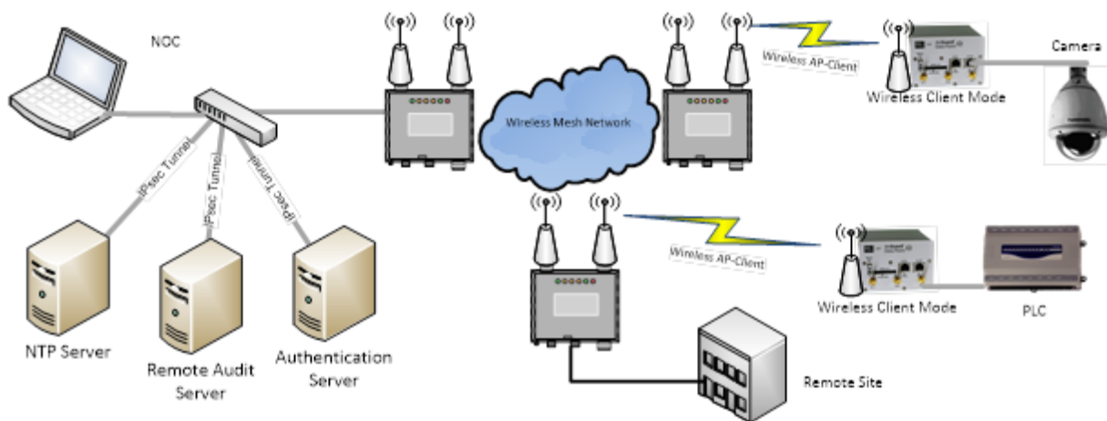
Figure 1: Typical Deployment Diagram
