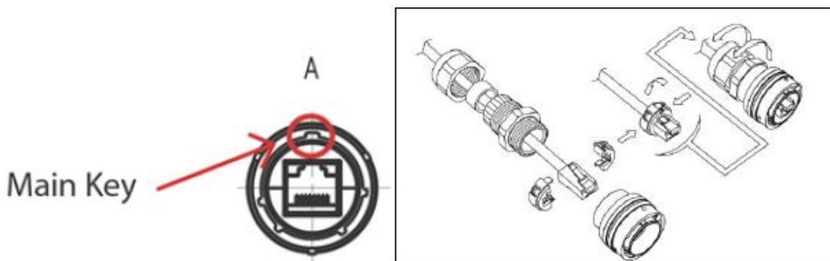
Figure 103: 3e-525N Ethernet Cable Assembly
