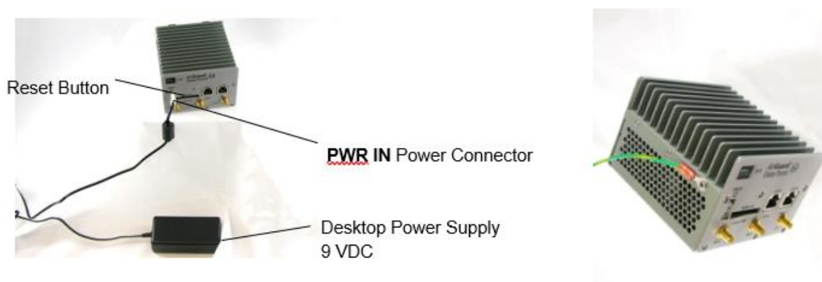
Figure 3: 3e-523N Power Supply and Ground Connections
