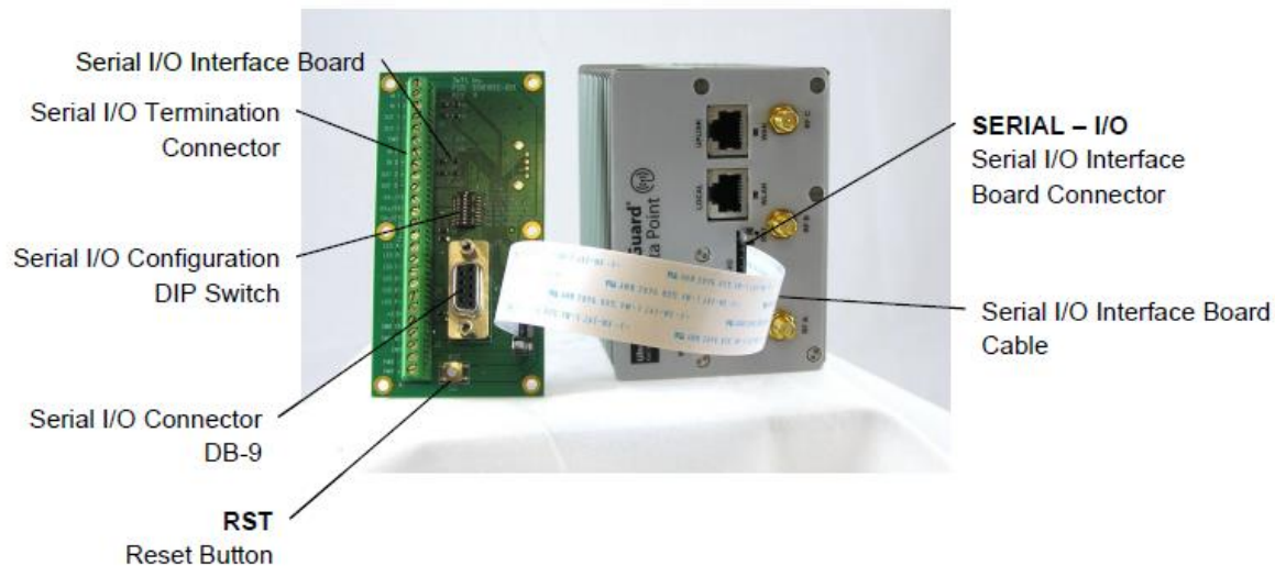
Figure 107: Serial I/O Interface Board
