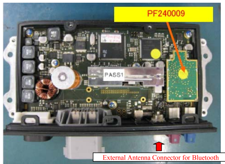
Fig 2. Top View of MAIN PWB that installed Bluetooth Module “PF240009”
