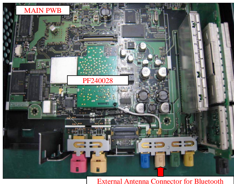
Fig 2. Top View of MAIN PWB that installed Bluetooth Module “PF240028”
