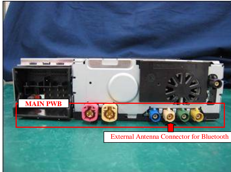
Fig 3. Rear view of Car audio that installed “PF240028” (Example)
