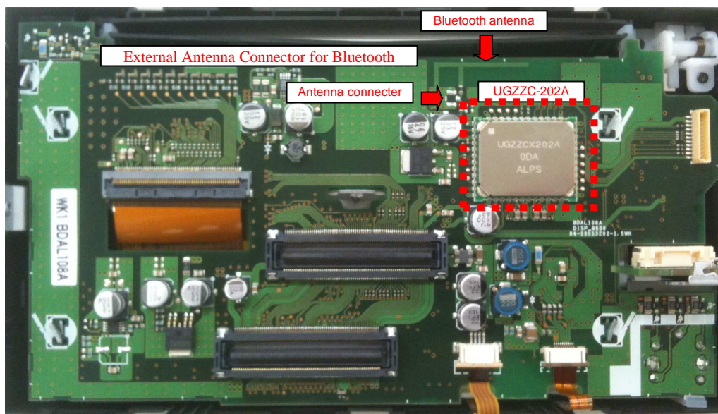
Fig 2. Reverse View of Display unit that installed Bluetooth Transmitter “UGZC-202A”
