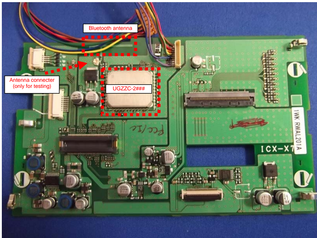
Fig 2. Top view of “ICS-X7 BT PWB”
