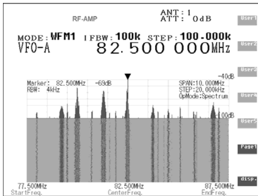
Waterfall Display
