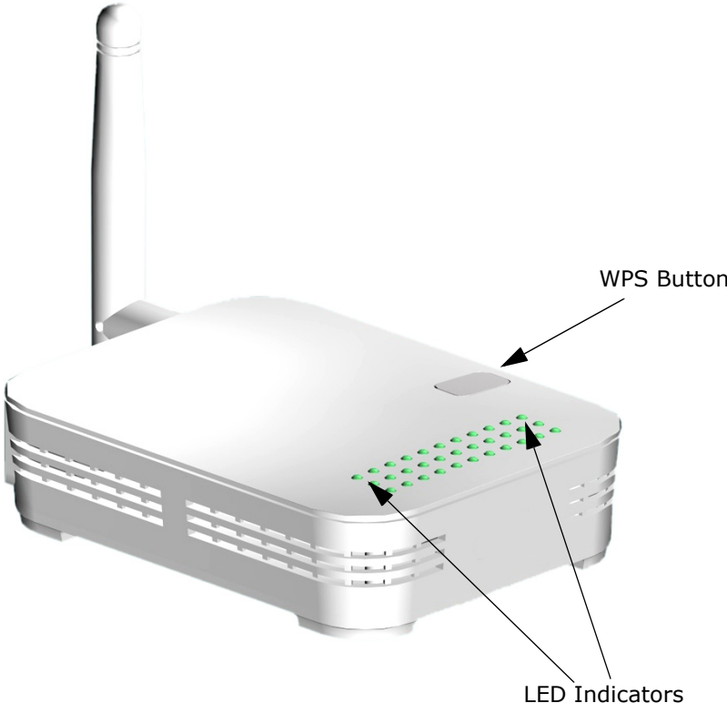
Figure 1: Top Panel
