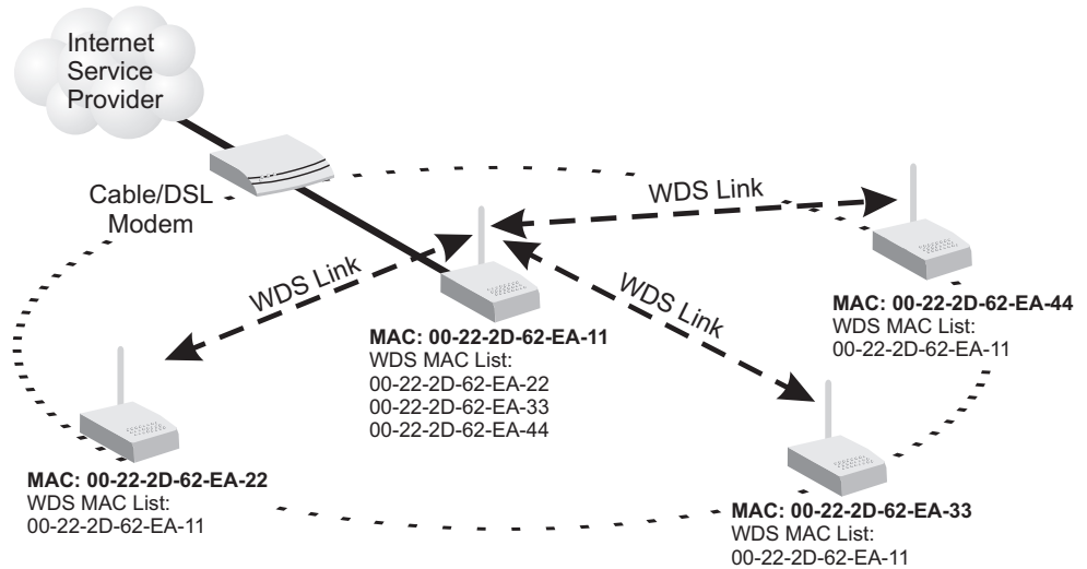
Figure 46: Manual WDS MAC Address Configuration
