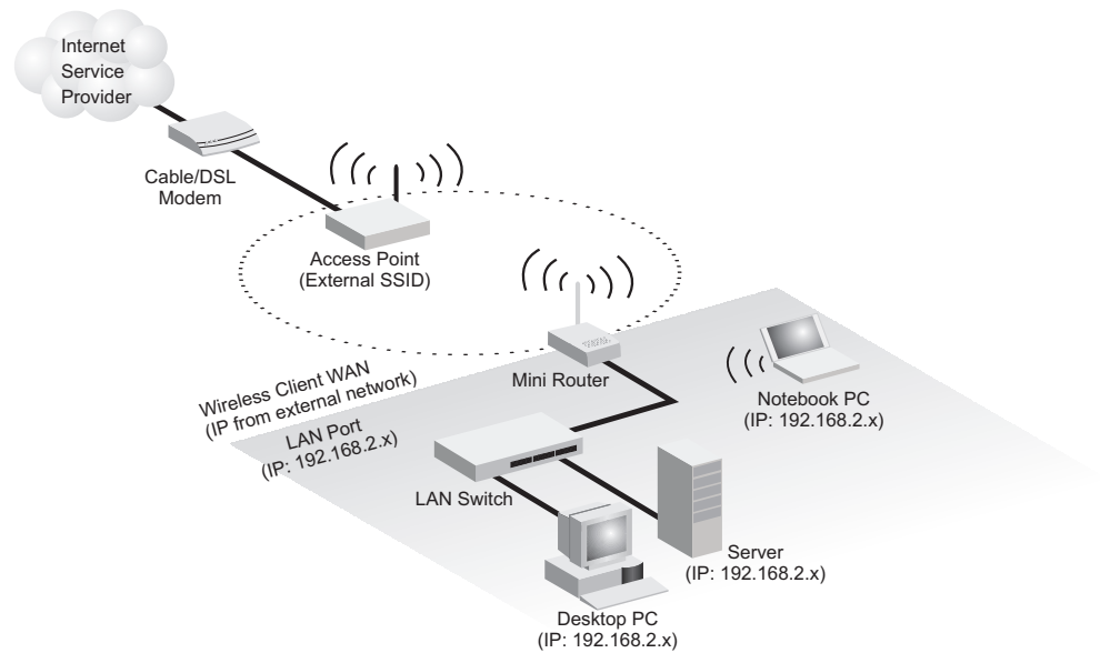
Figure 9: Operating as a Wireless Client
