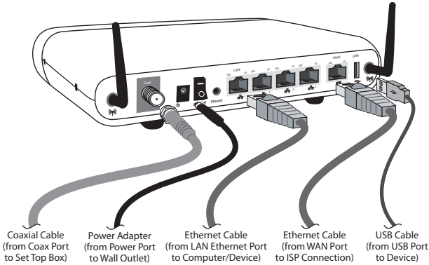
Rear view – Verizon FiOS Router (rev. F2)
