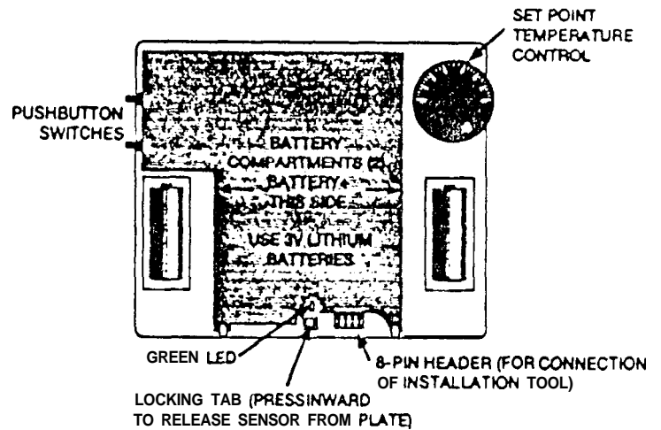
Figure 3. Wireless Sensor, Cover Removed
