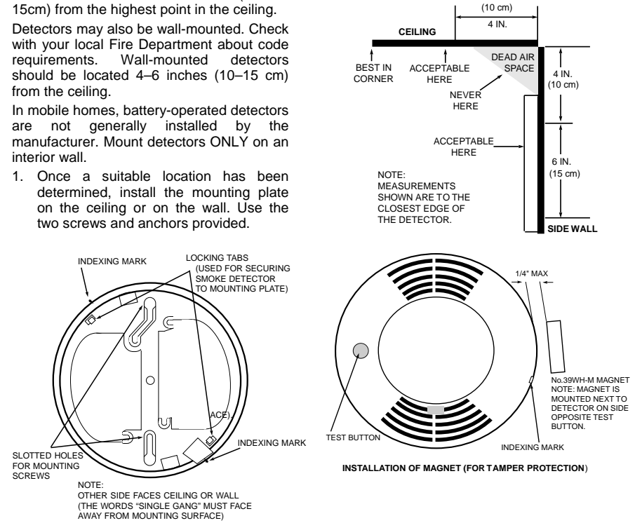
Figure 2. Mounting Details
