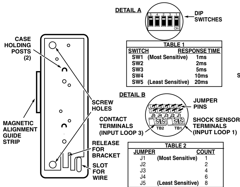
Diagram 1: MOUNTING PLATE
