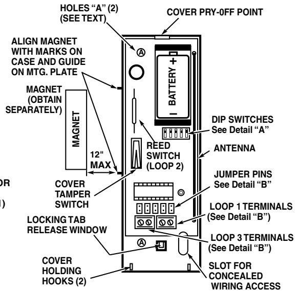
Diagram 2: 5819 (SHOWN WITH COVER REMOVED)
