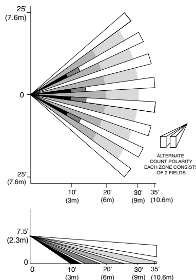
Figure 1. Protection Pattern
