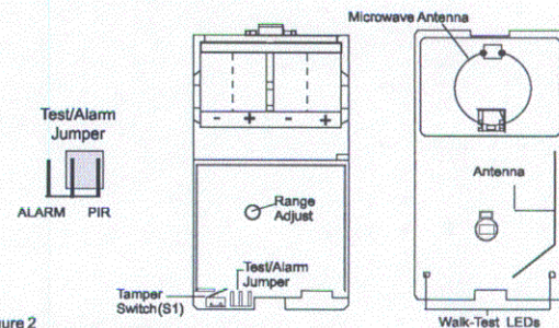
Figure 2 PCB Layout and Connections
