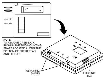
Figure 1 – Removing the 6150RF Case Back
