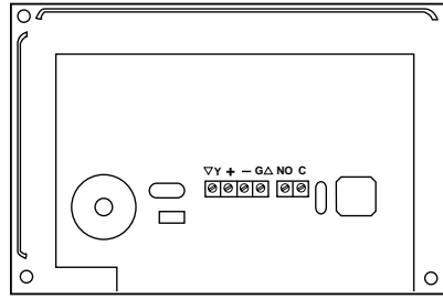
Figure 2 - 6150RF Wiring Connections
