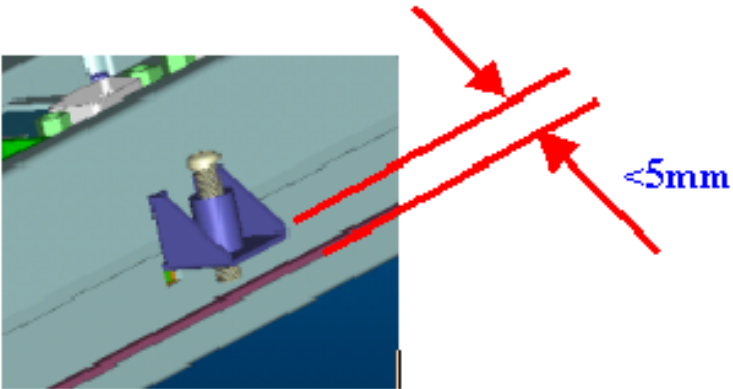
Figure 1.2: Panel Mounting
