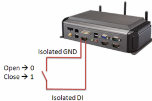
Figure 6.15 Digital in
