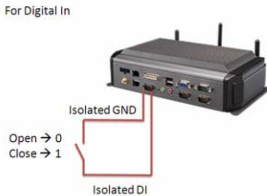
Figure 6.15 Digital in
