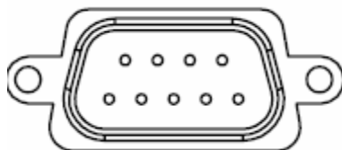
RS-232/RS-485/J1708 Connector
