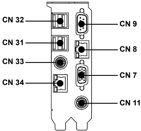
Figure 1.2: I/O Connectors
