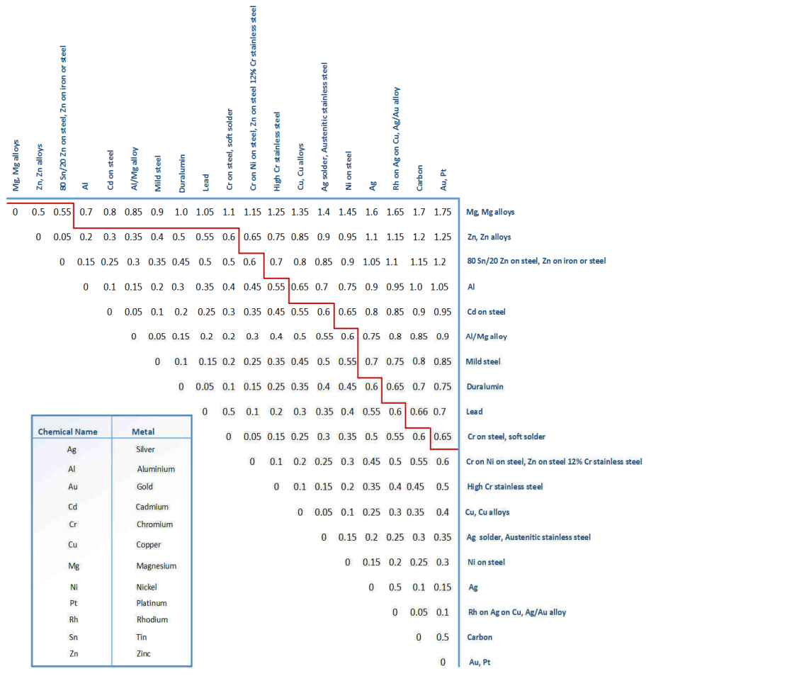
Figure 18: Recommended Metal Combinations
