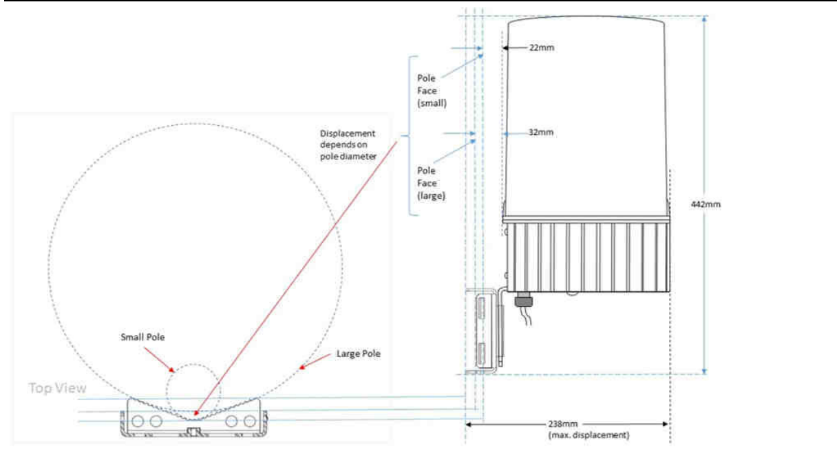
Figure 4: Product Dimension Envelope (Pole Mounted)
