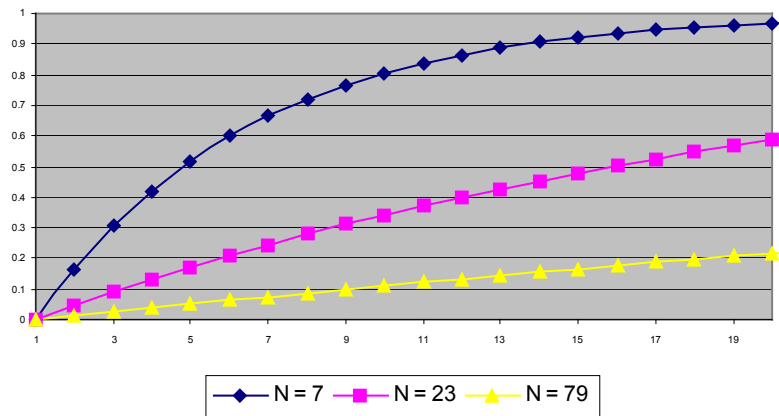
Figure 2-7: Hit probability as a function of active interferers
