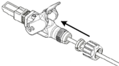
Figure 52: Insert Gland
