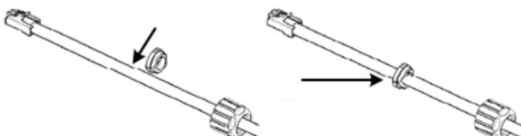
Figure 58: Insert Tightening Cone on Cable
