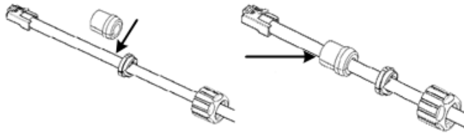
Figure 59: Insert Rubber Gland on Cable
