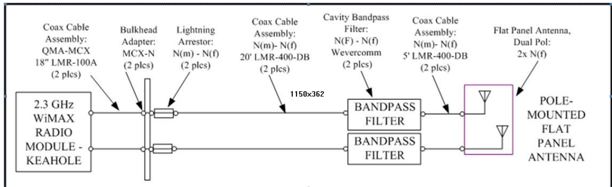
Figure 1 - Block Diagram
