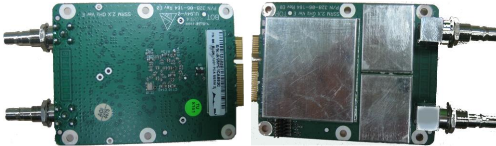
Figure 2 – SSRM PCIe module
