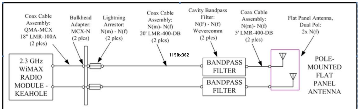
Figure 1 - Block Diagram
