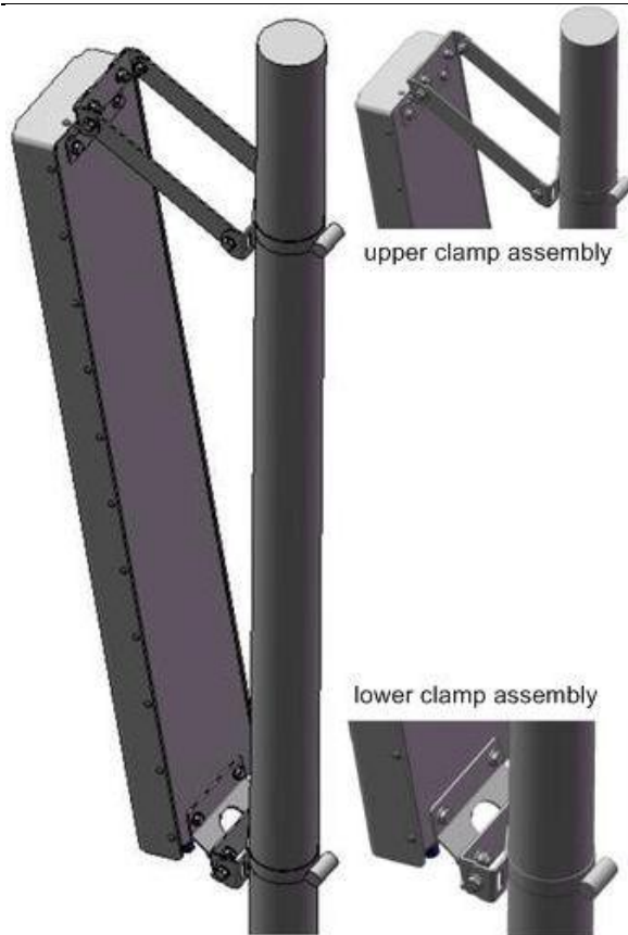
Figure 27 - Adjustable Mounting Kit, with Snaplock Stainless Steel Bands
