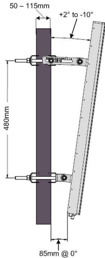
Figure 29 - Adjustable Mounting Kit 2, with 'V' Blocks
