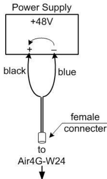
Figure 44 – DC Power connection
