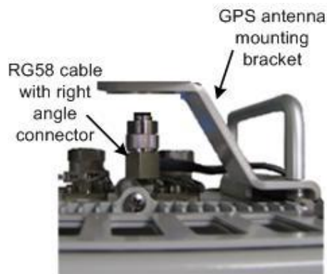
Figure 36 - GPS cable assembly prior to mounting
