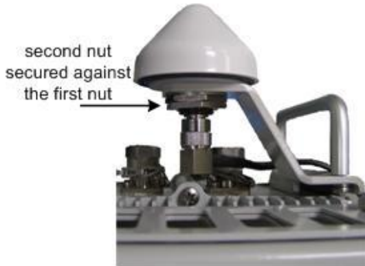
Figure 38 - GPS antenna assembled on bracket
