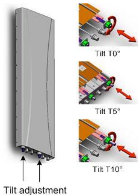
Figure 31 - Variable tilt antenna
