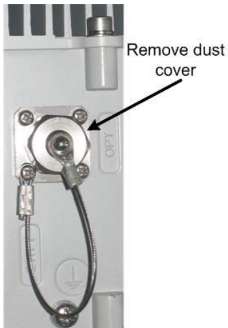
Figure 56 - fiber-optic connector with dust cover
