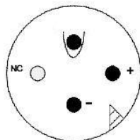
Figure 45 - Power connector – Air4G-W24 bottom panel
