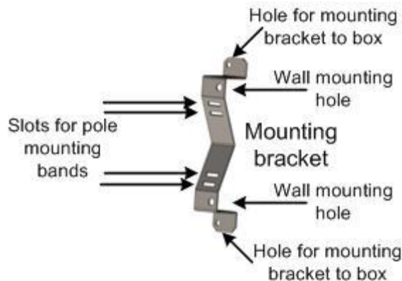
Figure 40 - mounting bracket (2 required)
