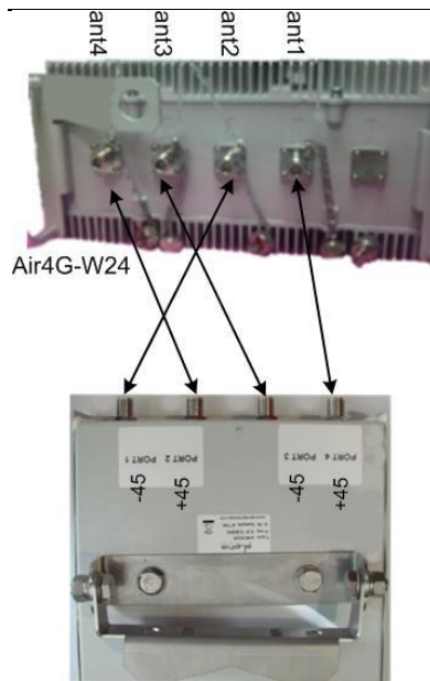
Figure 35 - Quad port antenna connection – 2
