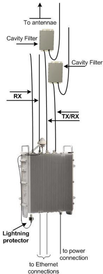
Figure 24 - Cavity filter(s) installation
