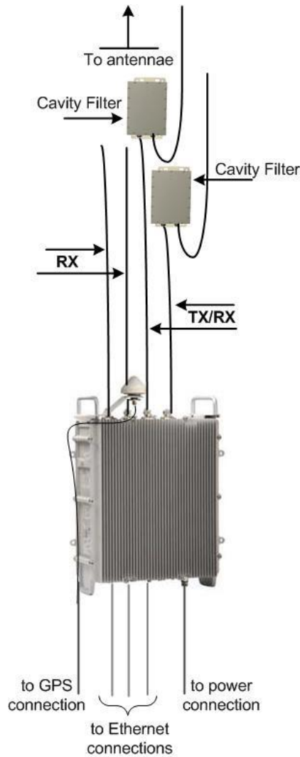
Figure 33 - Cavity filter(s) installation
