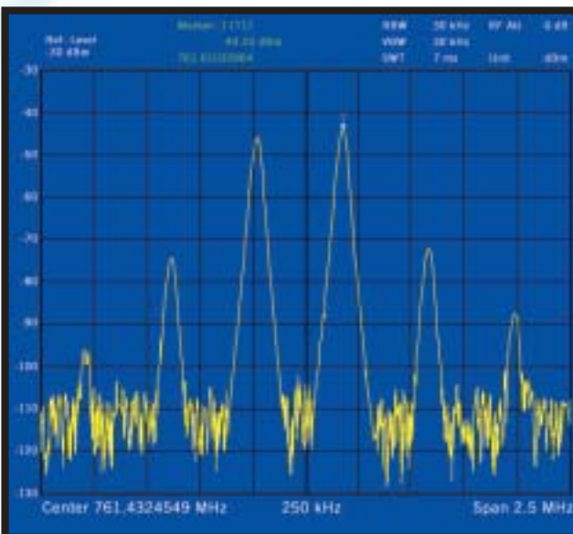
Intermodulation trace on a spectrum analyzer display Intermodulation products from 2 carrier frequencies, 3rd-order IMD and 5th-order IMD.
