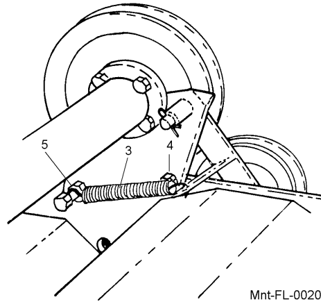
Inboard (Drive) Bearing - Figure Mnt-FL-0023 and Mnt-FL-0020.
