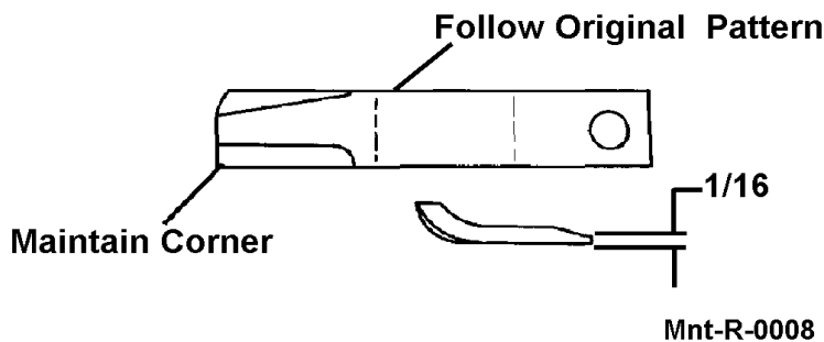
IMAGE 4. Blade Maintenance
