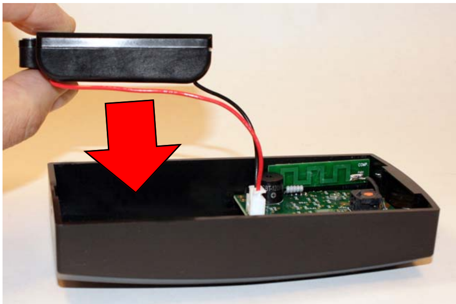
FIG. 18: INSTALL BATTERY PACK WITH FLAT SIDE UP
