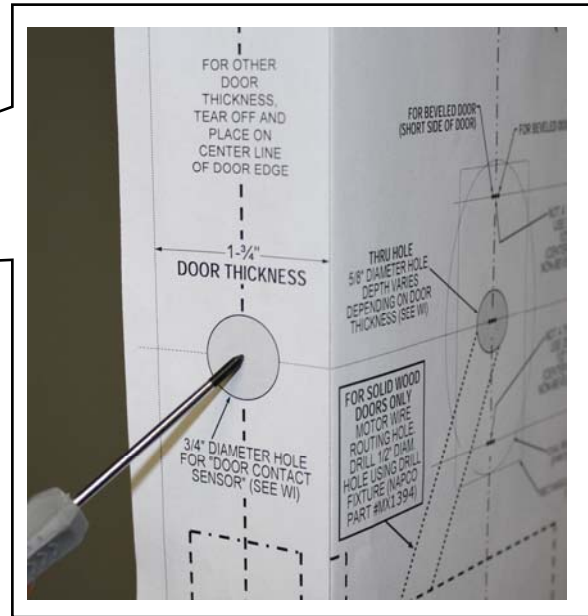
FIG. 5A: HOLE LOCATION DEPENDS ON DOOR THICKNESS
