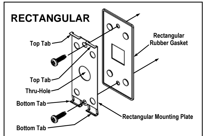
FIG. 15A: "RECTANGULAR PROXIMITY READER MOUNTING COMPONENTS"
