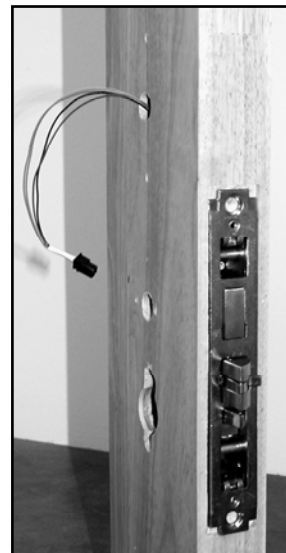
FIG. 12: ROUTE MORTISE LOCK WIRES THRU TO THE PROTECTED SIDE OF THE DOOR
