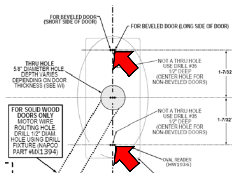
FIG. 9A: 7/64" PILOT HOLE ON OUTSIDE DOOR SURFACE FOR PROXIMITY READER
