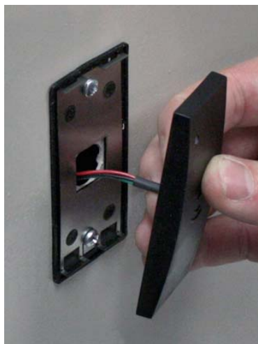
FIG. 15B: FEED THE WIRE INTO THE 5/8" DIAMETER THRU-HOLE (FROM "OUTSIDE" TO "INSIDE")
