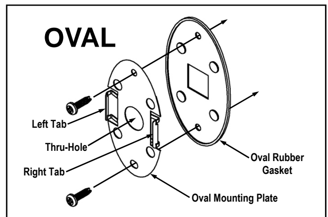
FIG. 14A: "OVAL MOUNTING PLATE" (WITH LEFT AND RIGHT "TABS") AND THE "OVAL RUBBER GASKET"
