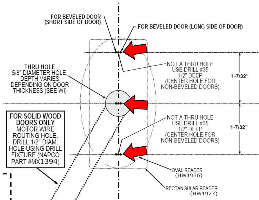
FIG. 4. EXAMPLE CLOSE UP OF WI2102 TEMPLATE FOR THE "PROXIMITY READER"
