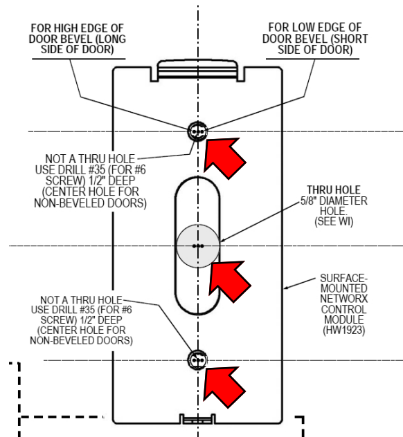
FIG. 8: MARK THE TWO "CONTROL UNIT MOUNTING PLATE" HOLES (ARROWS)
