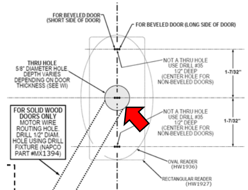
FIG. 9C: 5/8" DIAMETER THRU-HOLE
