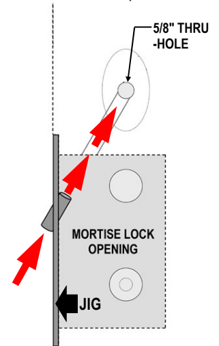
FIG. 11: SIDE VIEW: DRILL JIG (N9511DJ) DRILL HOLE INSIDE DOOR
