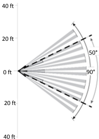
Figure 2. Top View: PIR Lens Coverage
