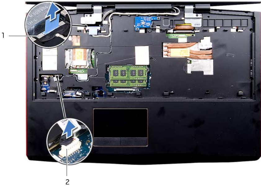
1 display-cable connector 2 LED logo-board cable
