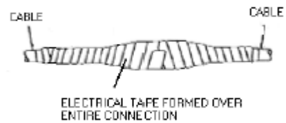
FIGURE 3 ELECTRICAL TAPE WRAPPED TIGHTLY AGAINST CABLE JACKET, TYPICAL BOTH ENDS
