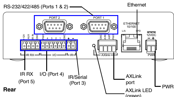
FIG. 2 NI-700 rear connectors and components
