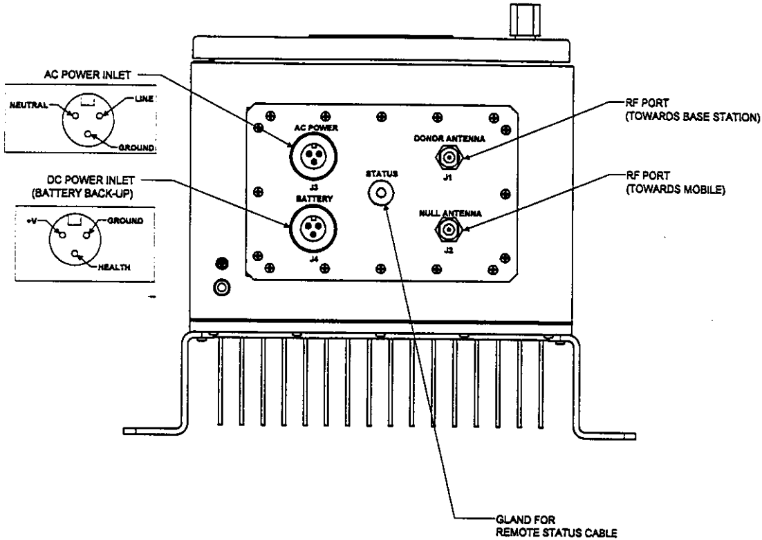
Figure 1-3 SelectAmp Connector Panel
