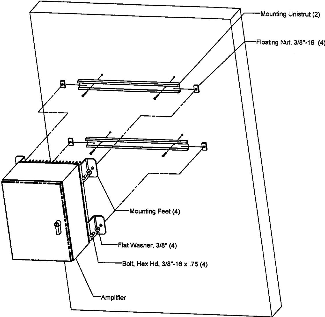
Figure 1 Wall Mounting
