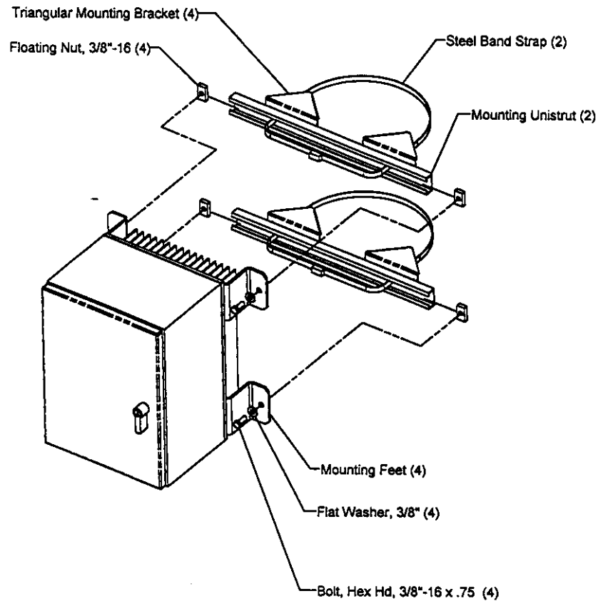
Figure 2 Pole Mounting
