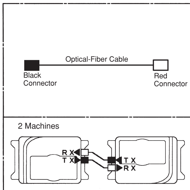
FIG. 8.2 Communication Cable Connection Diagram
