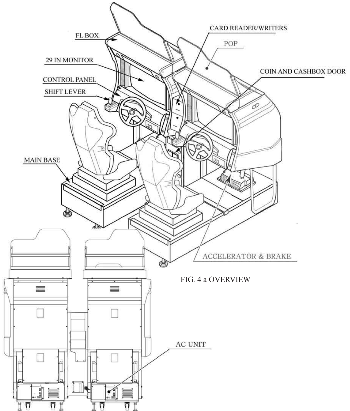
FIG. 4 b REAR VIEW
