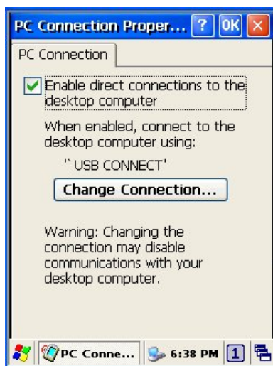
Figure 8-17 PC Connection
