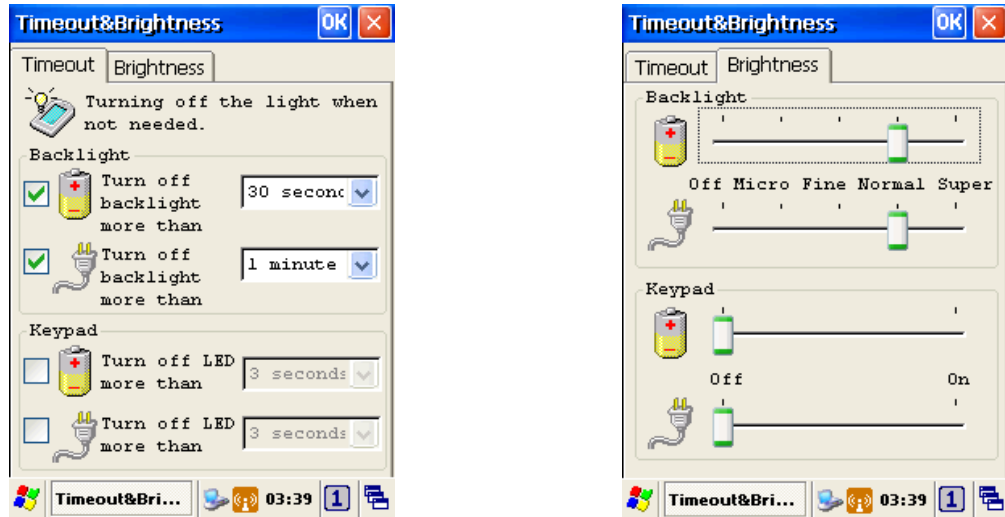
Figure 5-3 Timeout & Brightness
