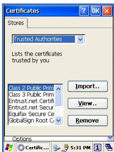
Figure 8-6 Certificates
