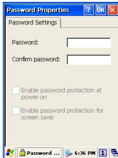
Figure 8-16 Password Properties
