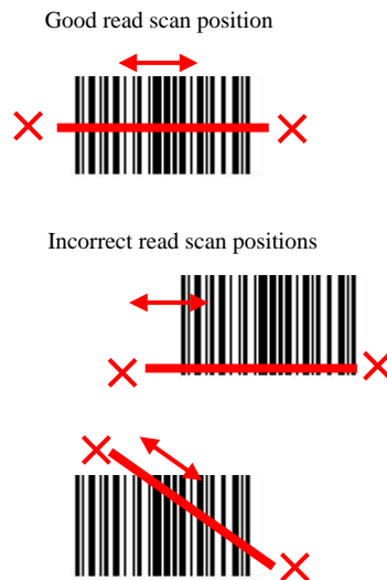
Figure 4-4 Scan Test
