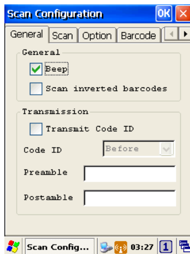
Figure 4-1-2 Scan Configuration
