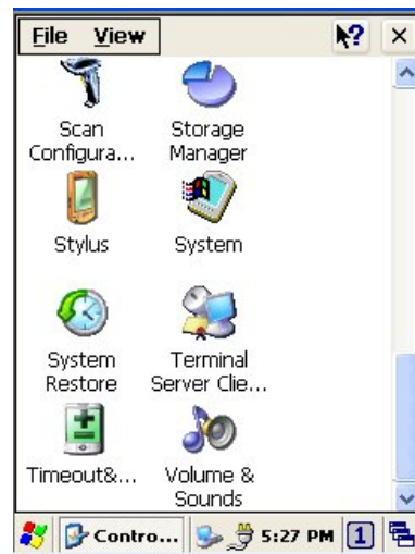
Figure 8-5-3 Control Panel
