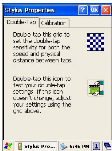
Figure 8-21 Stylus Properties
