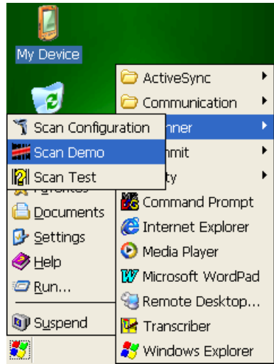
Figure 4-2-1 Scan Demo
