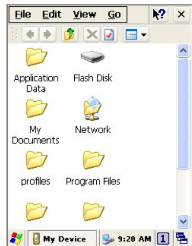
Figure 6-7 Windows Explorer
