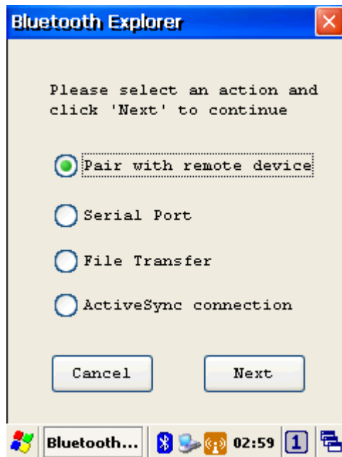
Figure 3-18 Bluetooth Explorer
