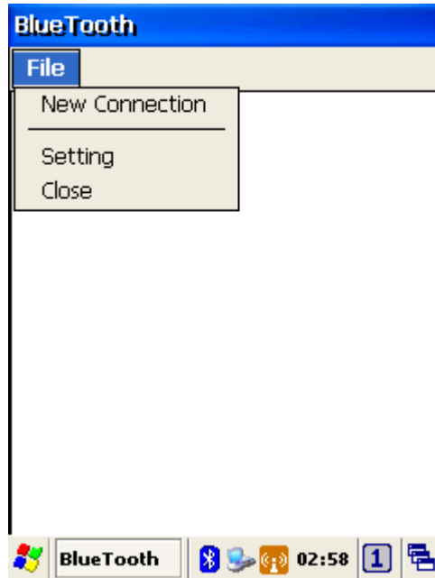
Figure 3-17 Bluetooth connection
