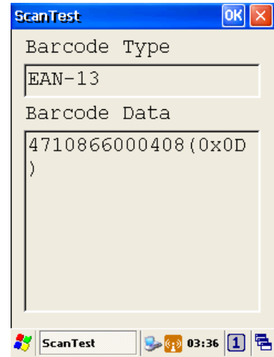
Figure 4-3-2 Scan Test
