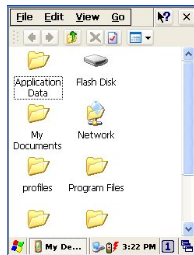
Figure 8-2 My Device
