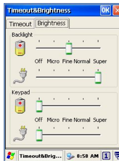
Figure 3-10 Timeout & Brightness
