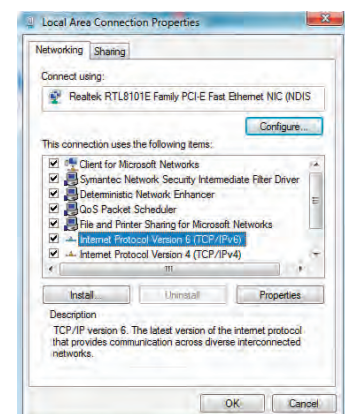
TCP/IPv6 Selected
