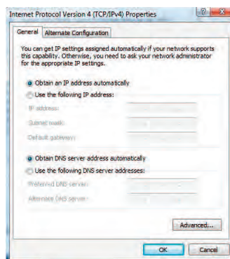
TCP/IPv4 Properties
