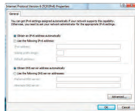
TCP/IPv6 Properties
