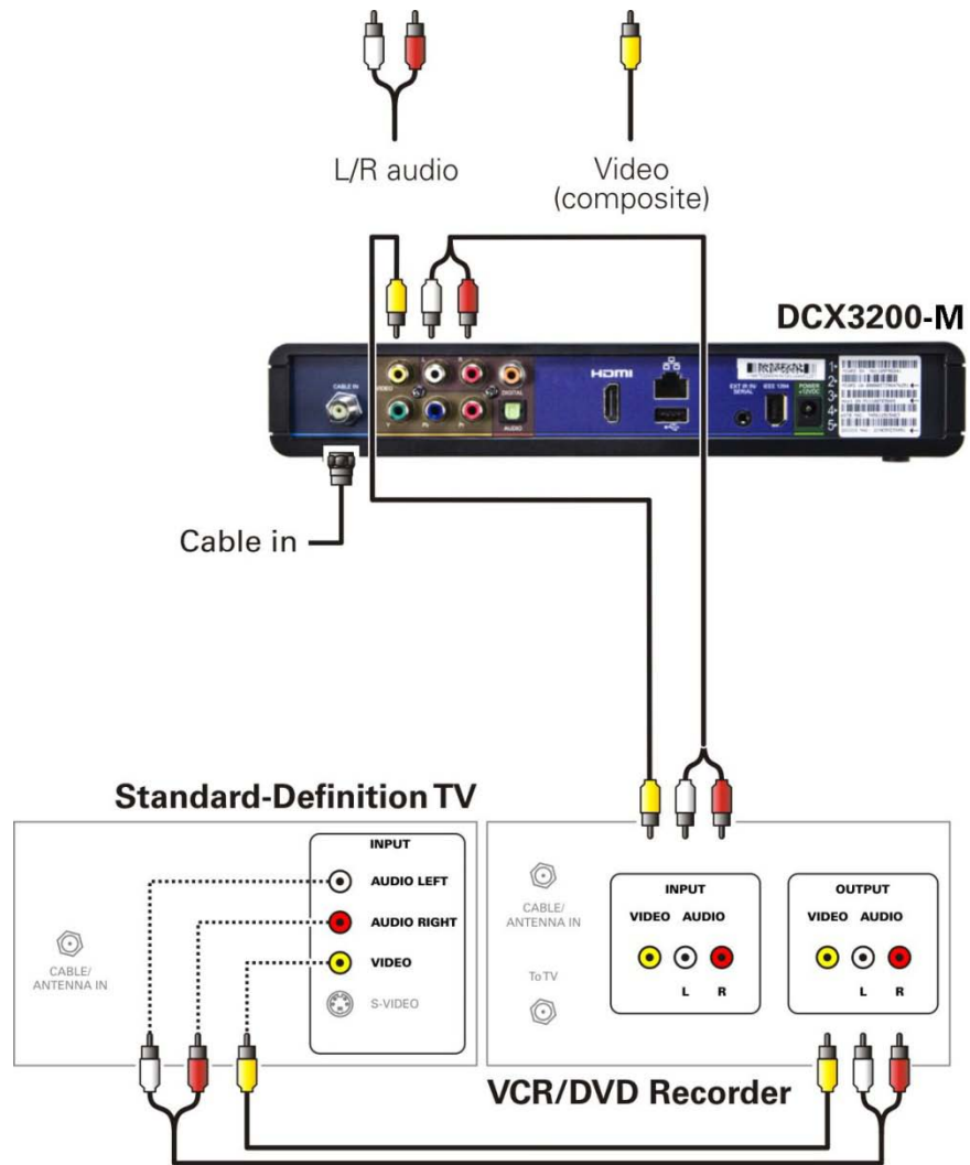
Figure 8: Connecting an SDTV and VCR/DVD Recorder
