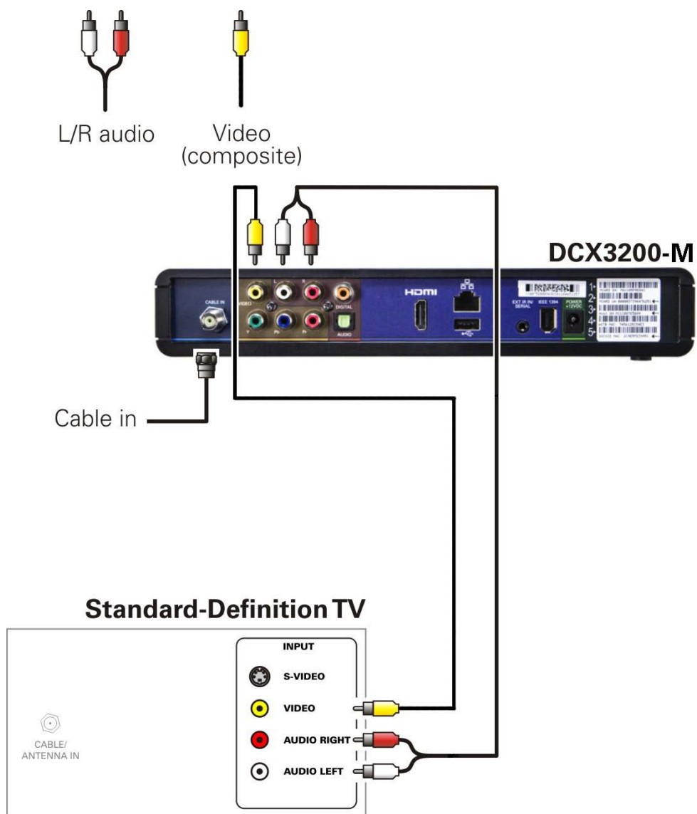
Figure 7: Connecting an SDTV
