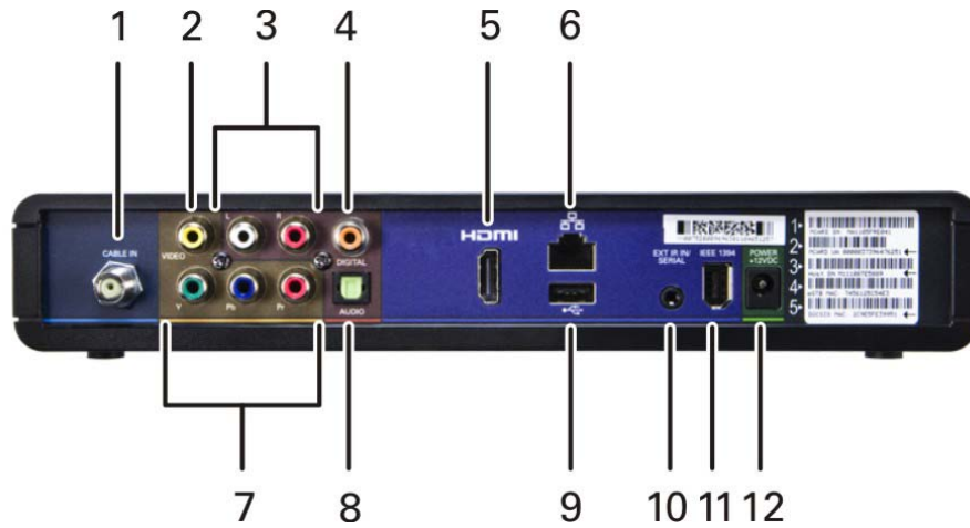
Figure 2: Rear Panel
