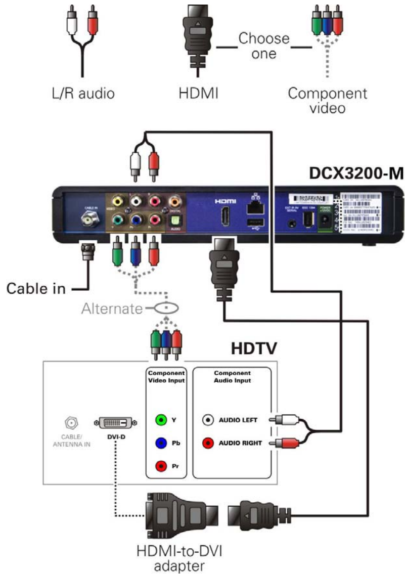
Figure 4: Connecting an HDTV – Separate Video/Audio Connections
