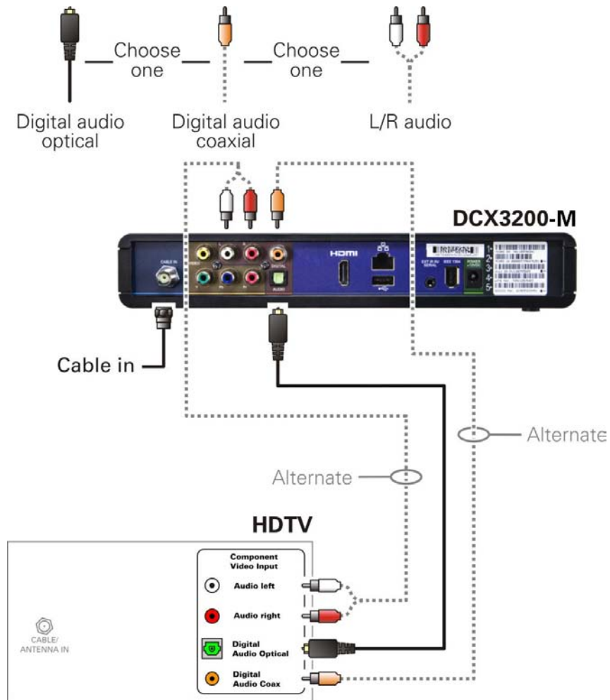
Figure 5: Connecting to an HDTV – Alternate Audio Connections
