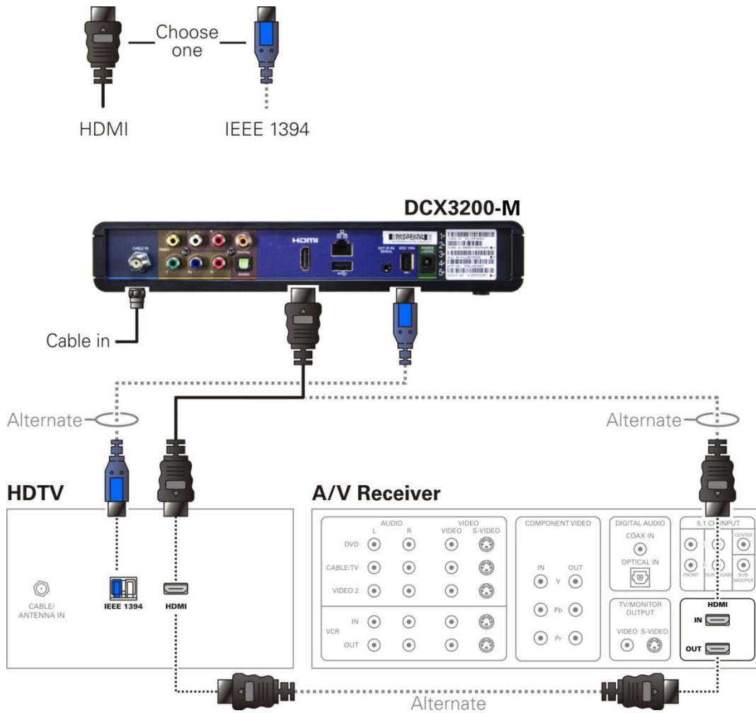
Figure 3: Connecting an HDTV — Single Connection for Video/Audio
