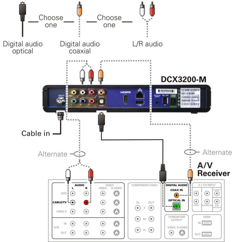
Figure 6: Connecting an A/V Receiver – Audio
