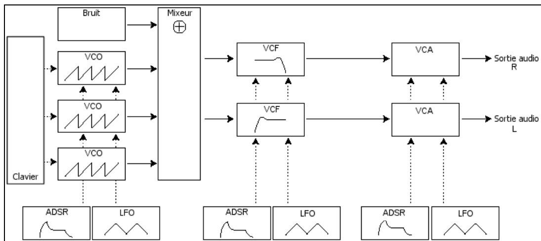
Synthesizer scheme
