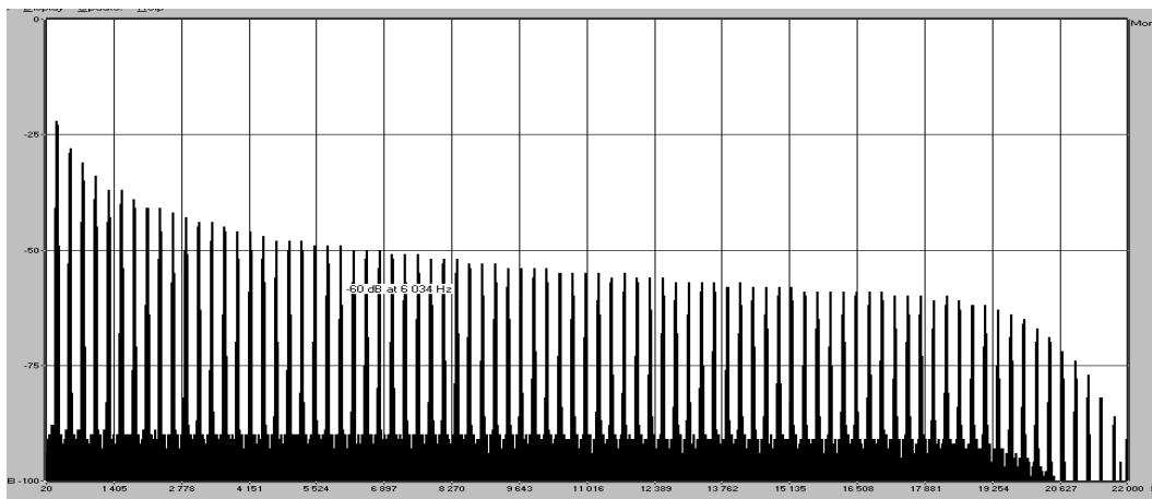
Linear frequency spectrum of the Moog Modular V oscillator made with TAE®
