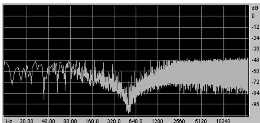
Band-reject filter
