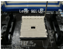
STEP 1: Lift Up The Socket Lever
