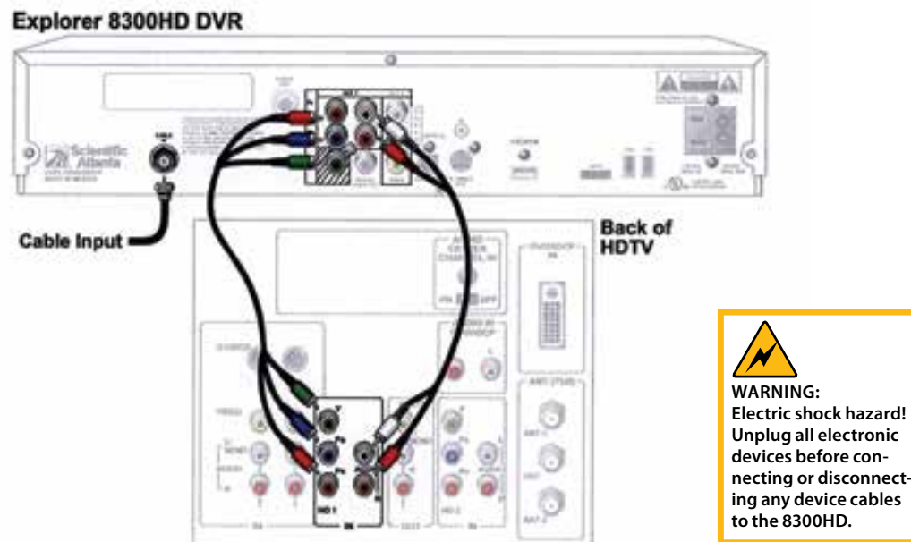
Diagram 1. Connecting the 8000 or 8300 HD-DVR using component connection
