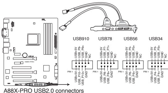
A88X-PRO USB2.0 connectors
