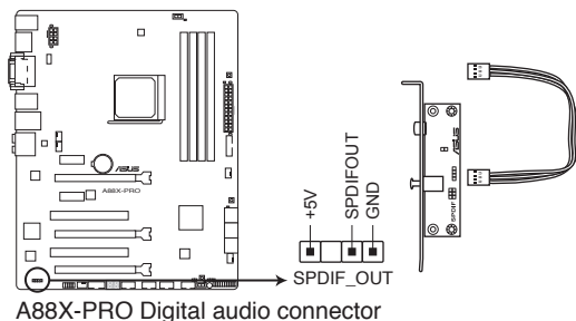
A88X-PRO Digital audio connector
