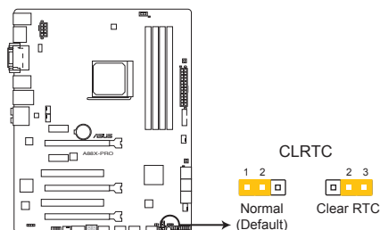
A88X-PRO Clear RTC RAM
