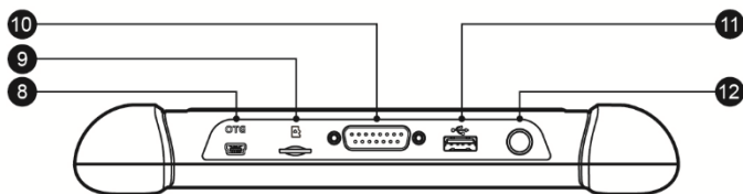
Figure 2-0-3 MaxiCheck MX808 Display Tablet Top View
