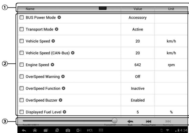
Figure 6-0-13 Sample Data Playback Screen
