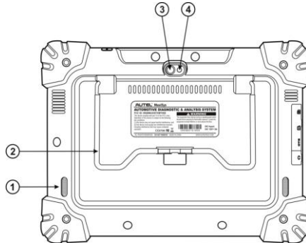
Figure 2-2 MaxiSys Back View
