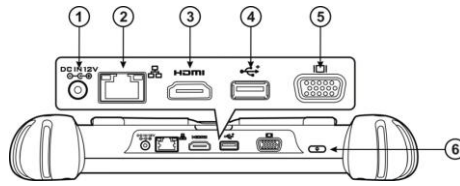
Figure 2-4 MaxiSys Top View
