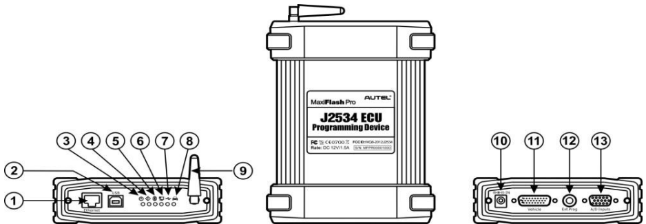
Figure 2-6 J2534 ECU Programming Device
