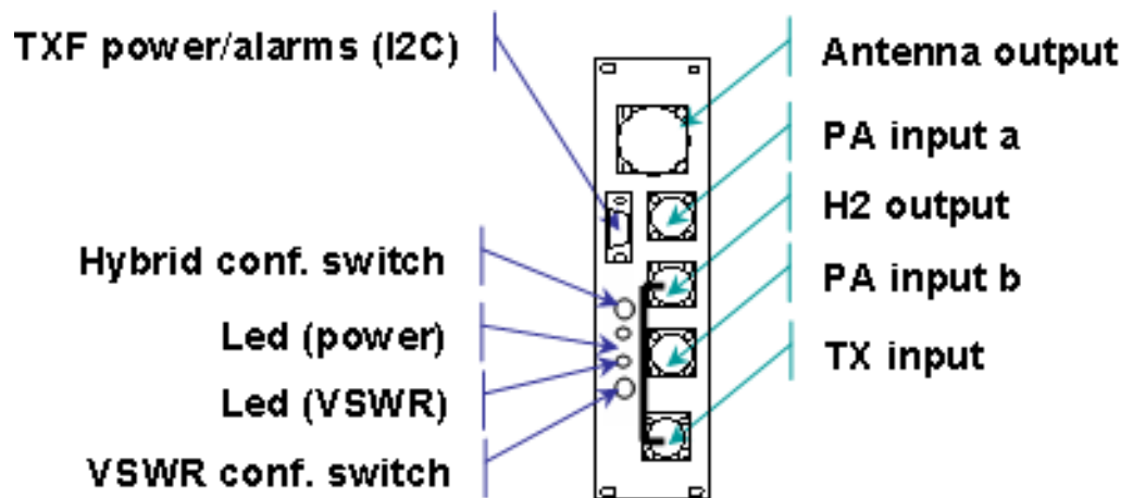
Figure 3-12 TXF front panel (with H2 coupling option)
