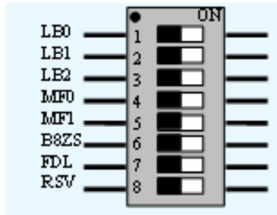
Figure 3-6 ICM Abis switch
