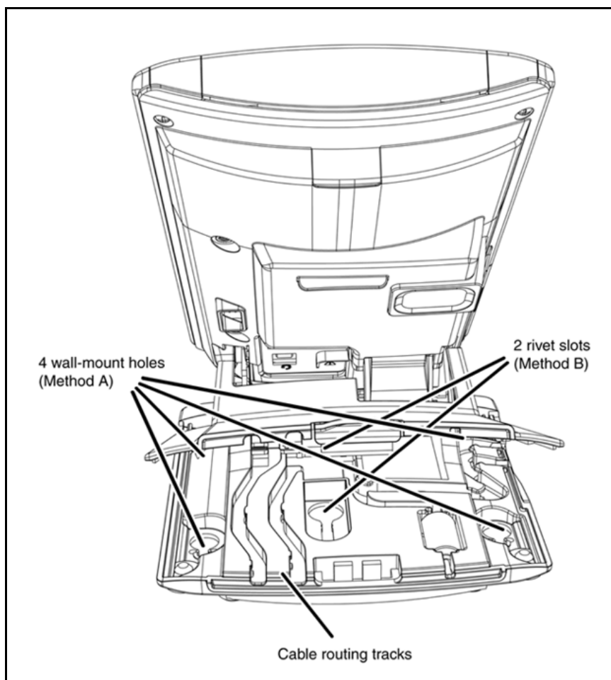
Figure 6: Cable routing tracks
