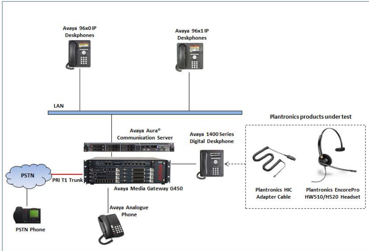
Figure 1: Avaya 1400 Series Digital Deskphones with Plantronics EncorePro HW510/HW520 Headsets and Plantronics HIC Adapter Cable
